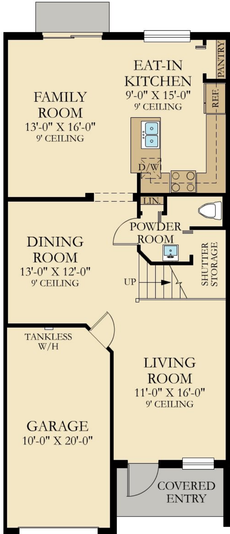
FIRST FLOOR
